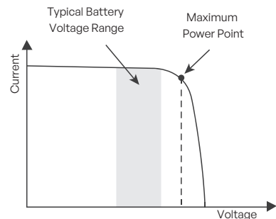
Current-Voltage (I-V) Curve
